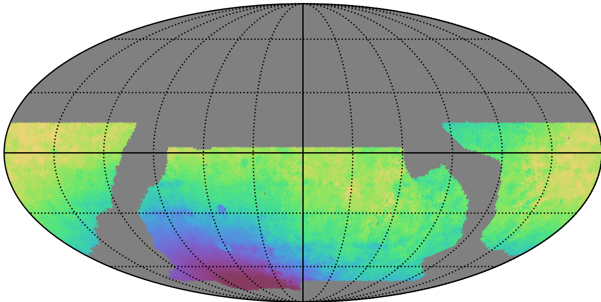
baseline_v2.0_10yrs WFD r band: Median solarElong
