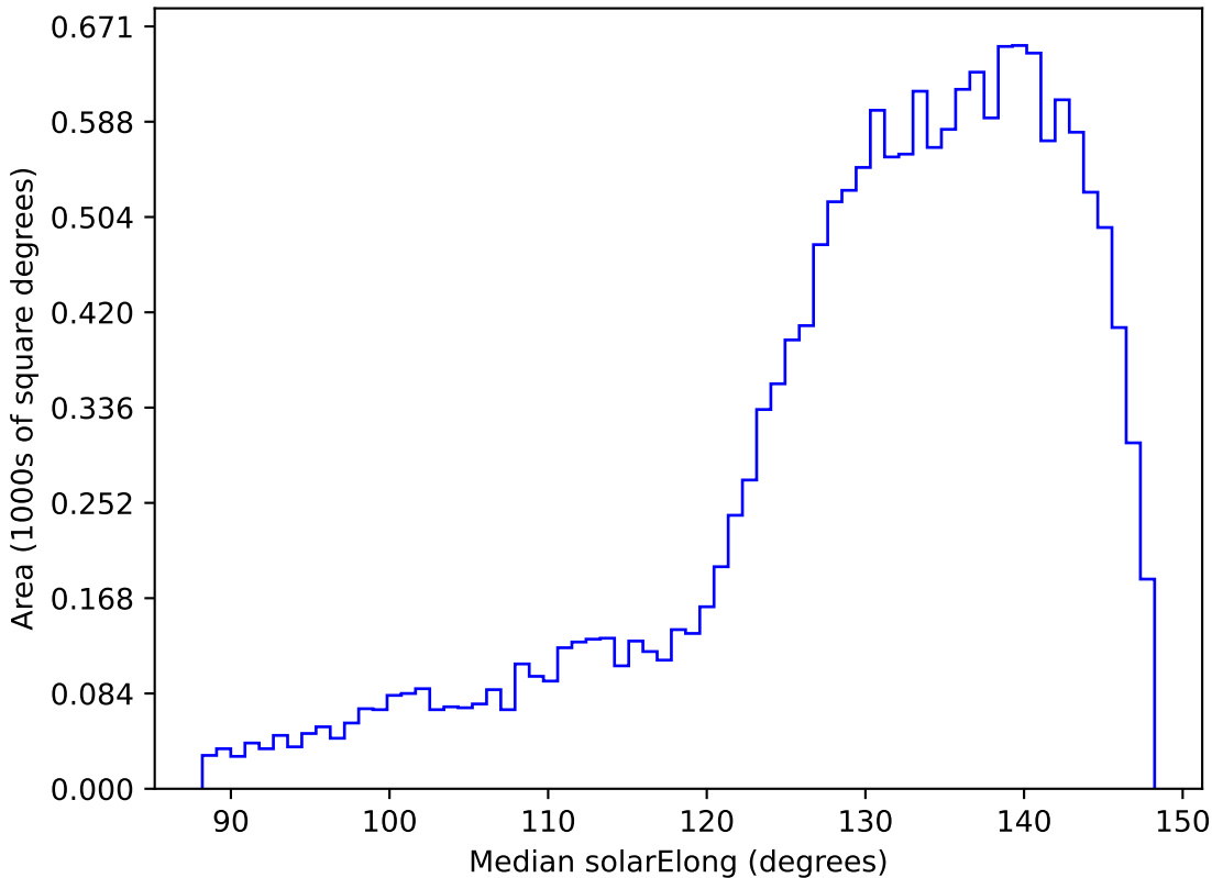
baseline_v2.0_10yrs WFD r band: Median solarElong
