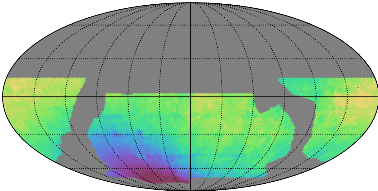
baseline_v2.0_10yrs WFD i band: Median solarElong
