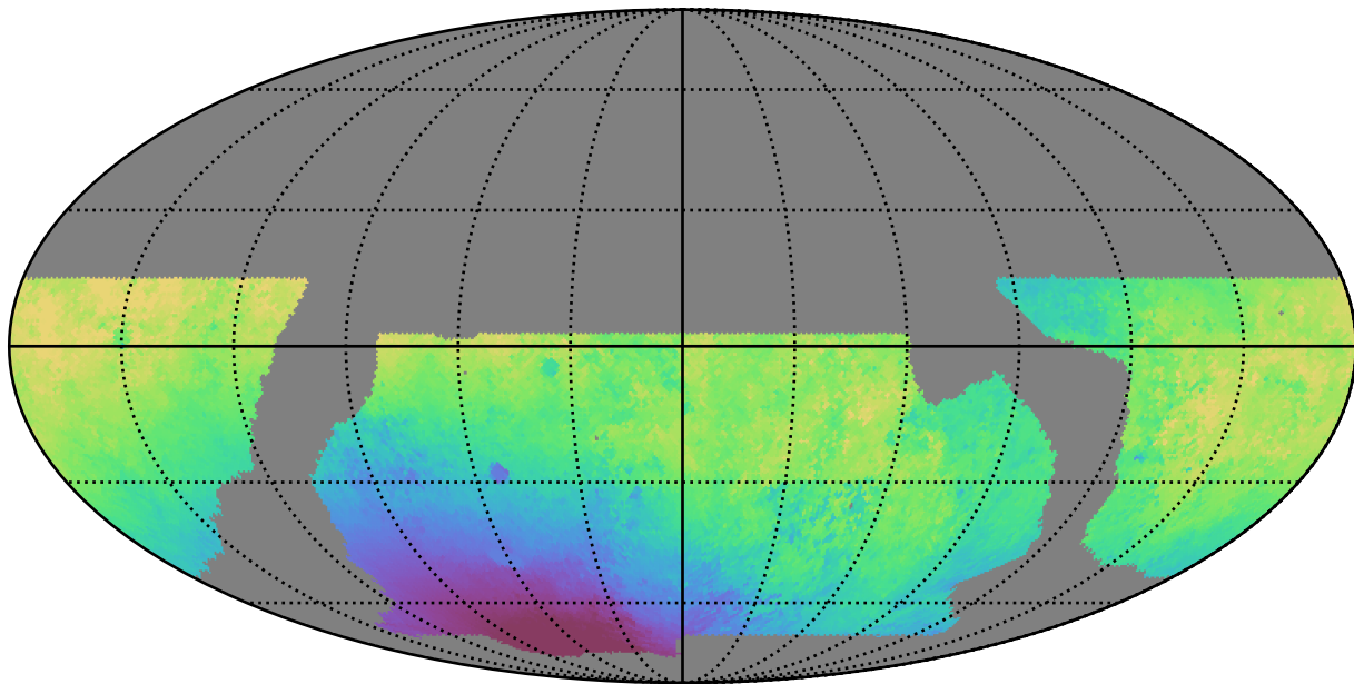
baseline_v2.0_10yrs WFD g band: Median solarElong
