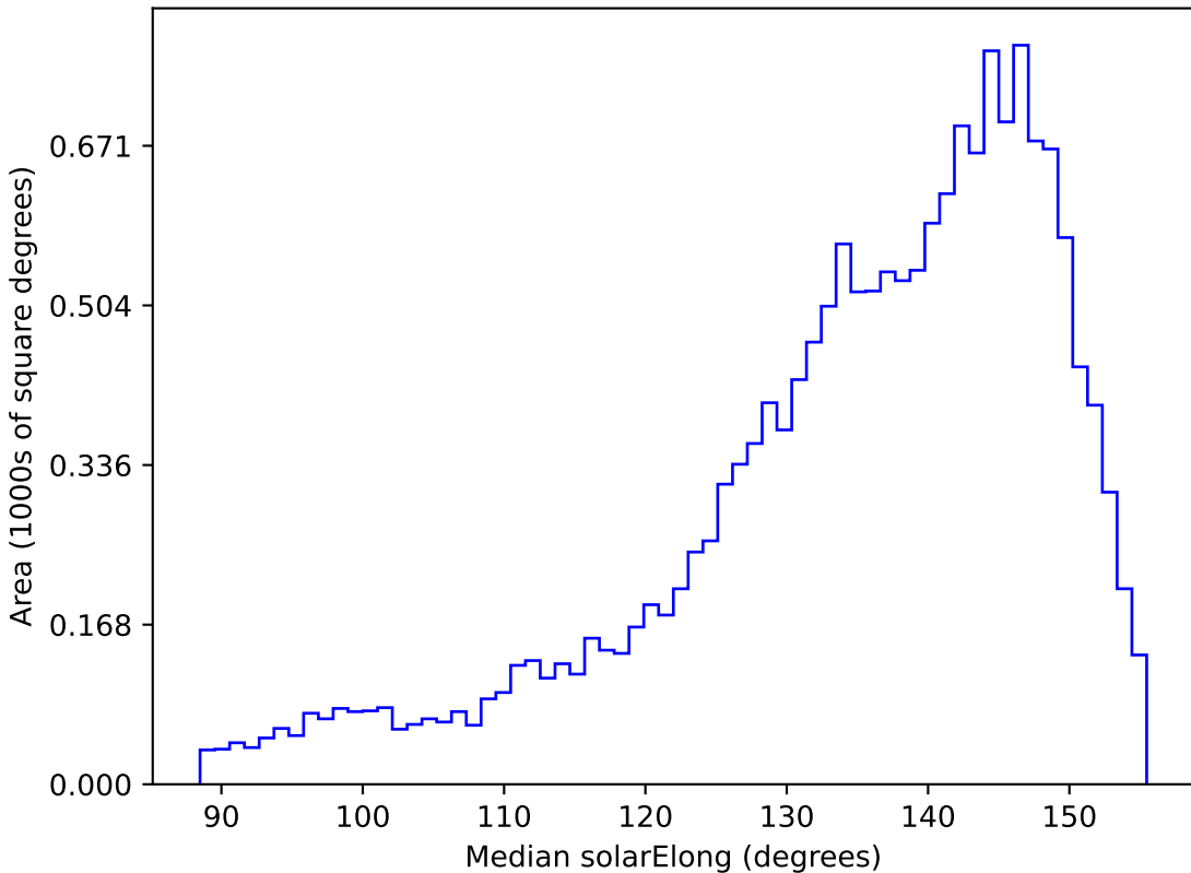
baseline_v2.0_10yrs WFD g band: Median solarElong
