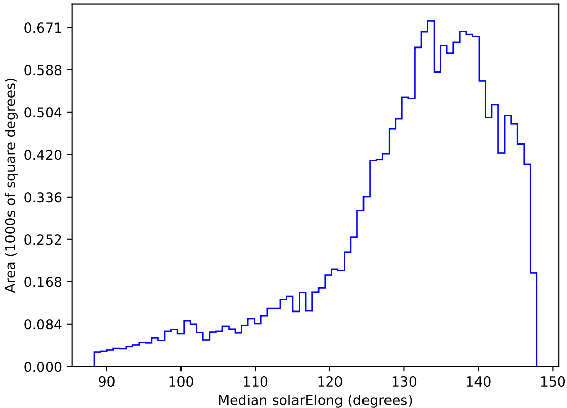
baseline_v2.0_10yrs WFD all bands: Median solarElong
