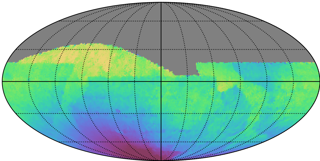
baseline_v2.0_10yrs All sky z band: Median solarElong
