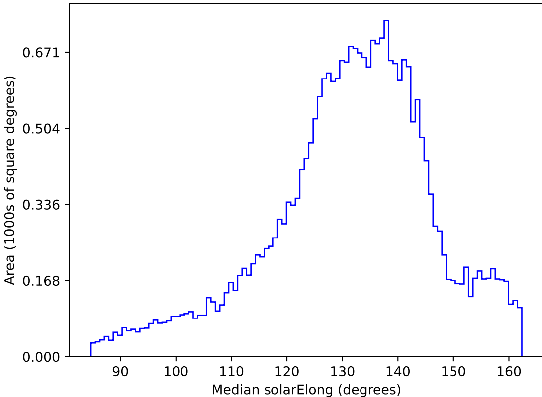
baseline_v2.0_10yrs All sky z band: Median solarElong
