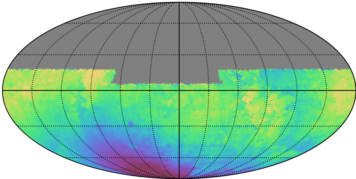
baseline_v2.0_10yrs All sky y band: Median solarElong
