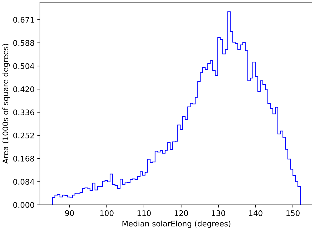
baseline_v2.0_10yrs All sky y band: Median solarElong
