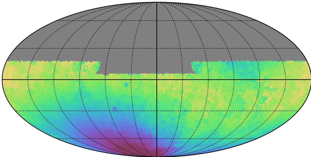
baseline_v2.0_10yrs All sky u band: Median solarElong
