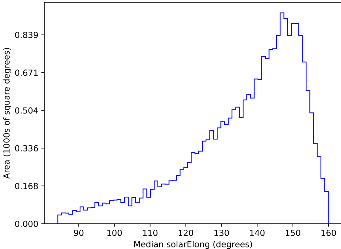
baseline_v2.0_10yrs All sky u band: Median solarElong
