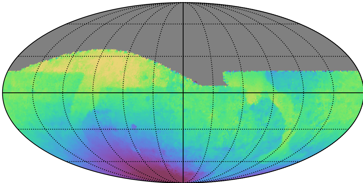
baseline_v2.0_10yrs All sky r band: Median solarElong
