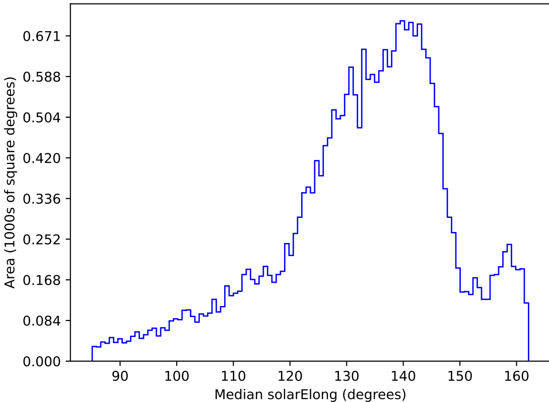
baseline_v2.0_10yrs All sky r band: Median solarElong
