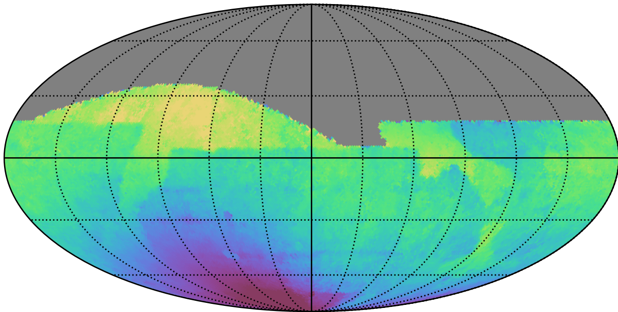
baseline_v2.0_10yrs All sky i band: Median solarElong
