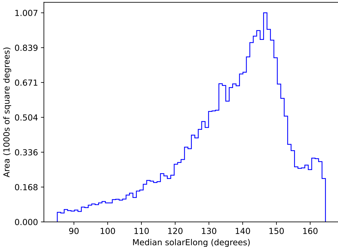
baseline_v2.0_10yrs All sky g band: Median solarElong
