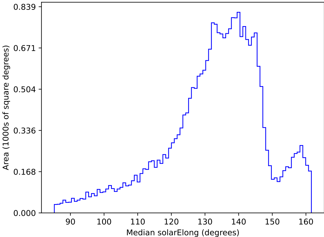
baseline_v2.0_10yrs All sky all bands: Median solarElong
