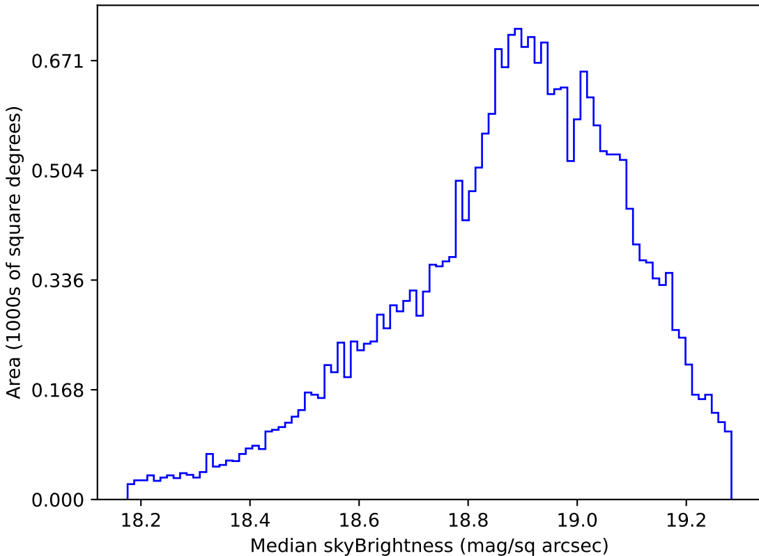
baseline_v2.0_10yrs Yr 1 z band: Median skyBrightness
