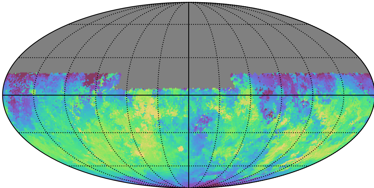
baseline_v2.0_10yrs Yr 1 y band: Median skyBrightness
