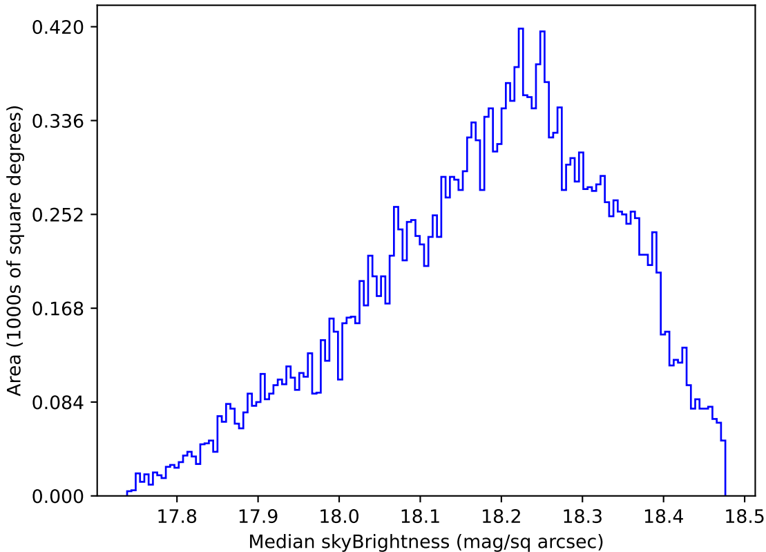
baseline_v2.0_10yrs Yr 1 y band: Median skyBrightness
