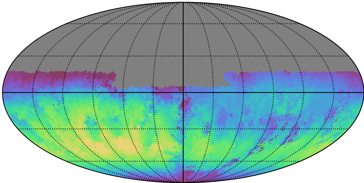
baseline_v2.0_10yrs Yr 1 u band: Median skyBrightness
