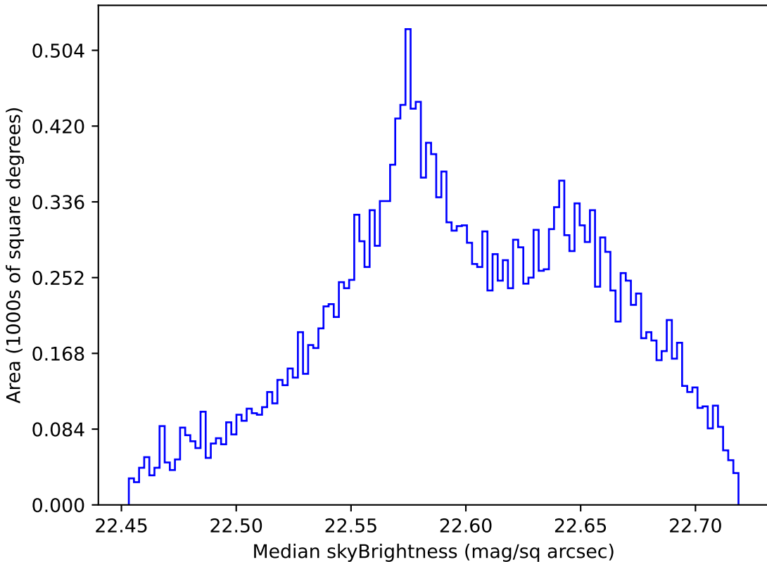
baseline_v2.0_10yrs Yr 1 u band: Median skyBrightness
