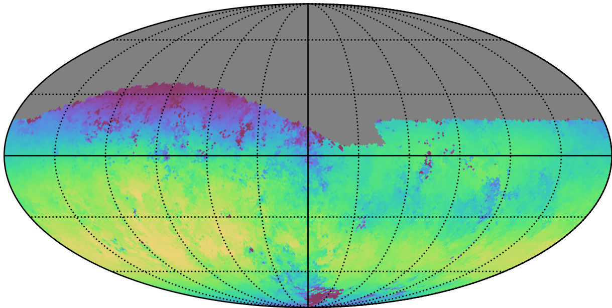
baseline_v2.0_10yrs Yr 1 r band: Median skyBrightness
