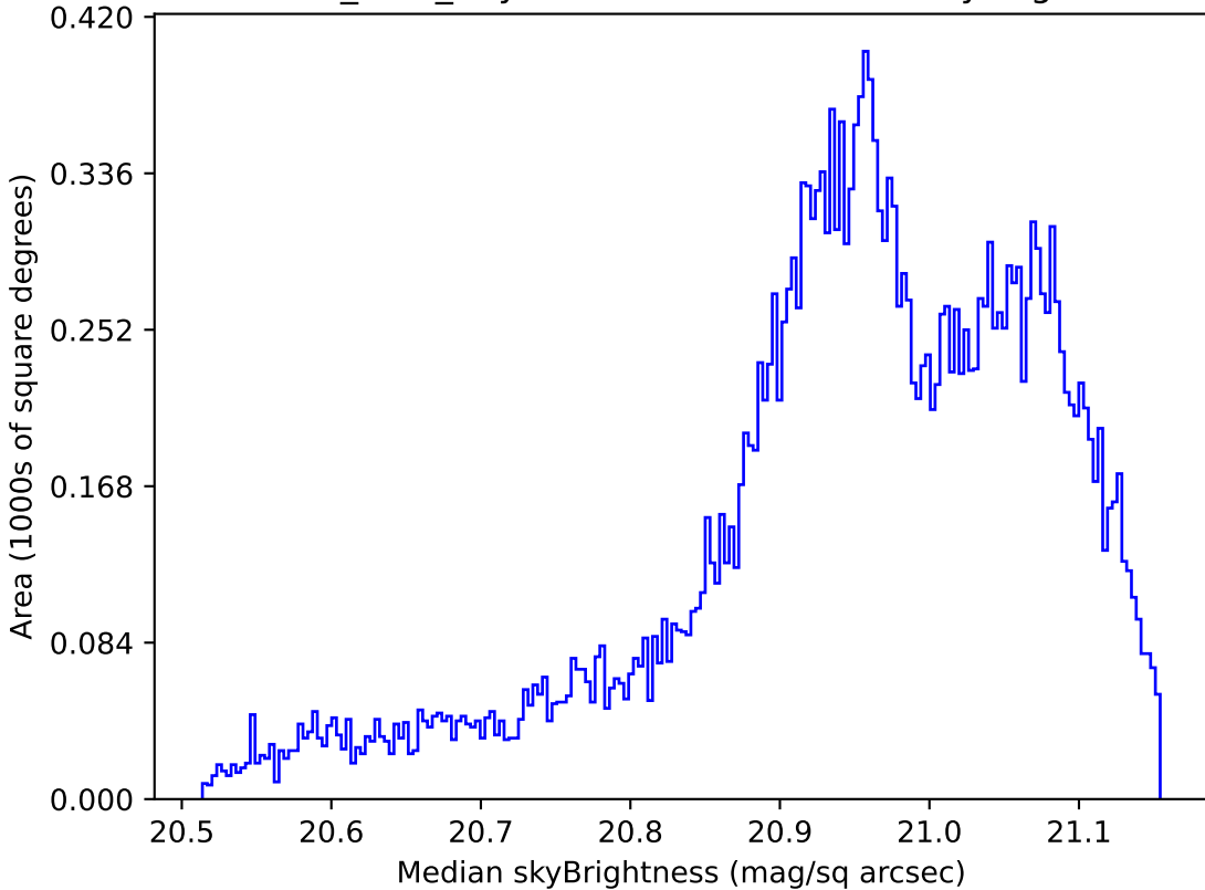
baseline_v2.0_10yrs Yr 1 r band: Median skyBrightness
