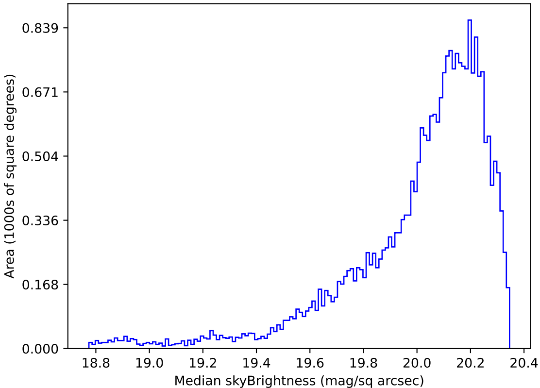
baseline_v2.0_10yrs Yr 1 i band: Median skyBrightness
