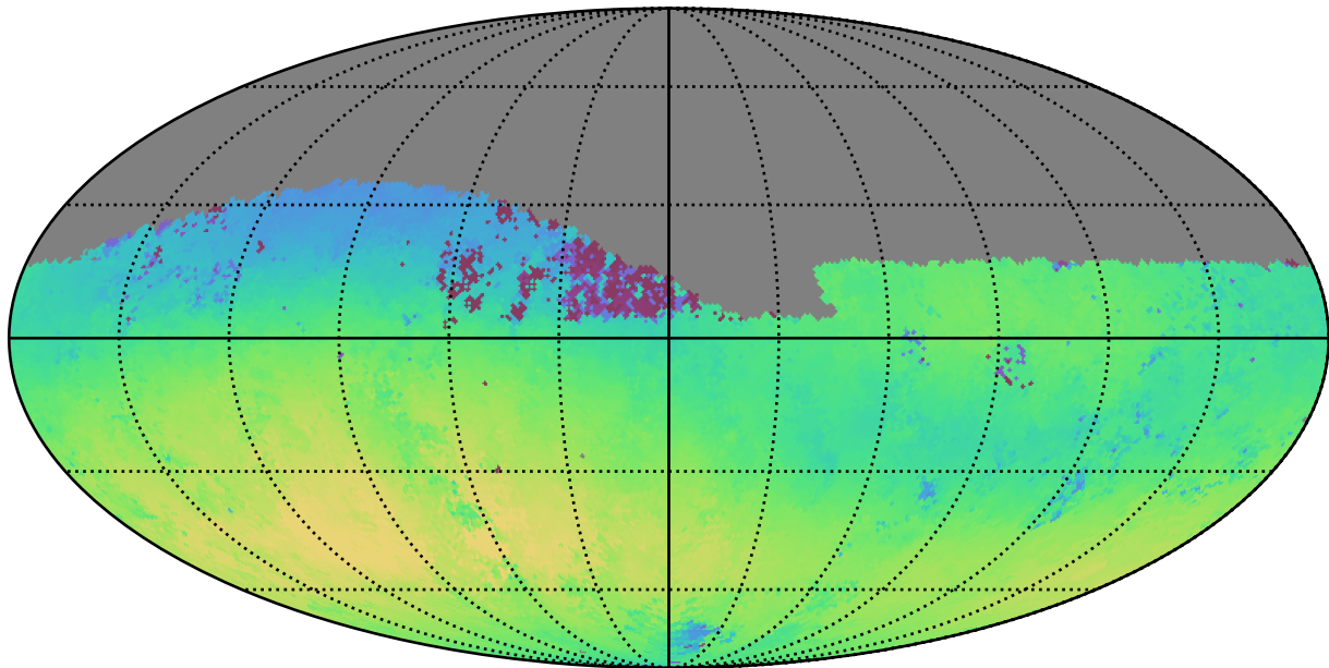
baseline_v2.0_10yrs Yr 1 g band: Median skyBrightness
