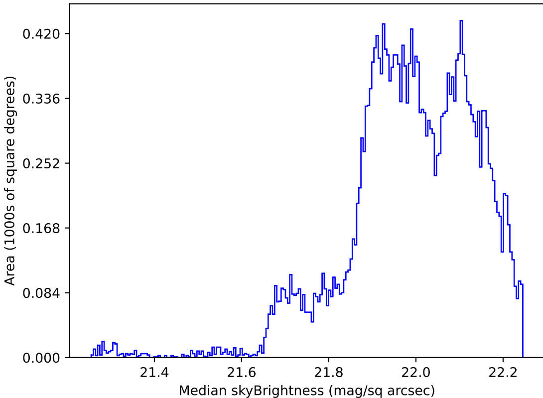
baseline_v2.0_10yrs Yr 1 g band: Median skyBrightness
