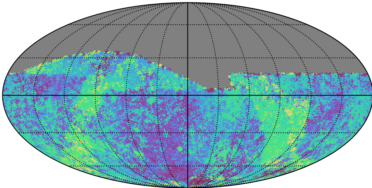
baseline_v2.0_10yrs Yr 1 all bands: Median skyBrightness
