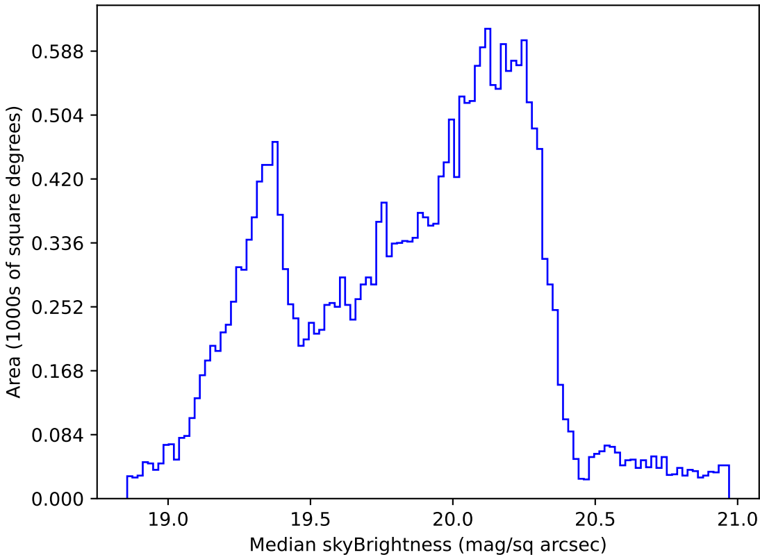
baseline_v2.0_10yrs Yr 1 all bands: Median skyBrightness
