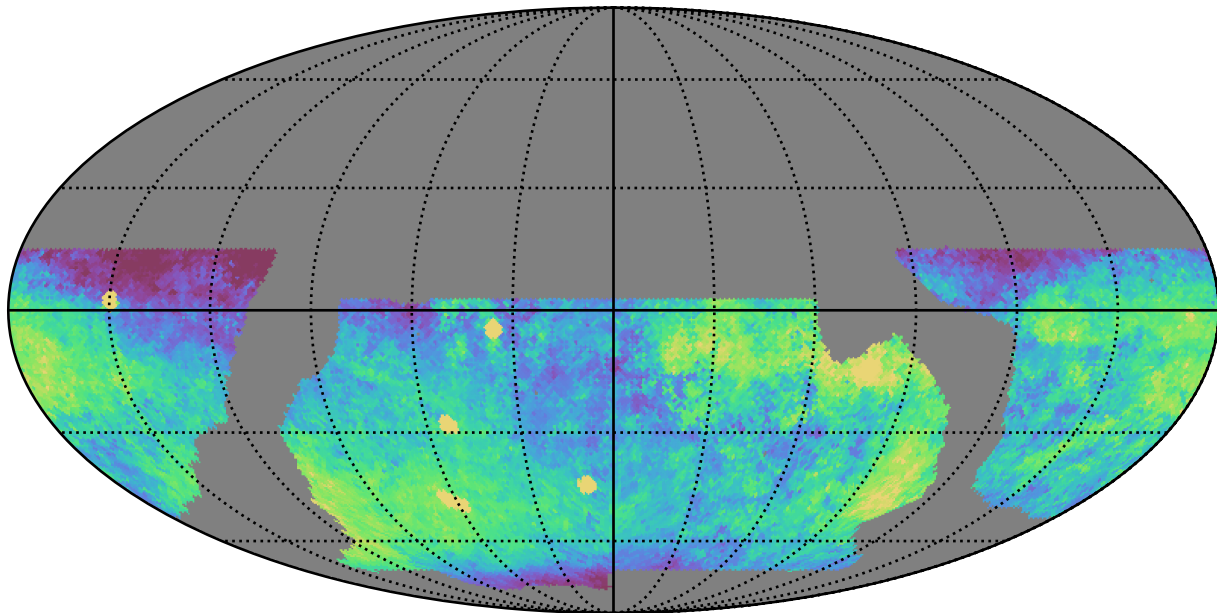
baseline_v2.0_10yrs WFD z band: Median skyBrightness
