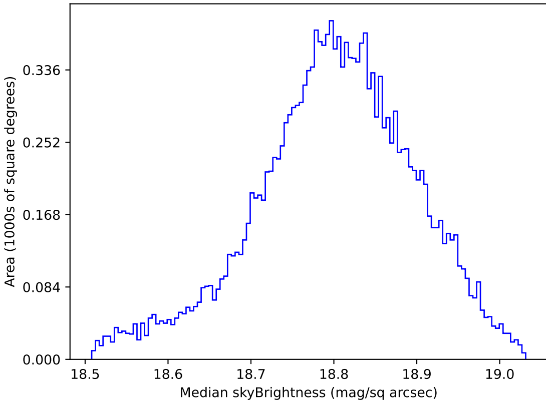
baseline_v2.0_10yrs WFD z band: Median skyBrightness
