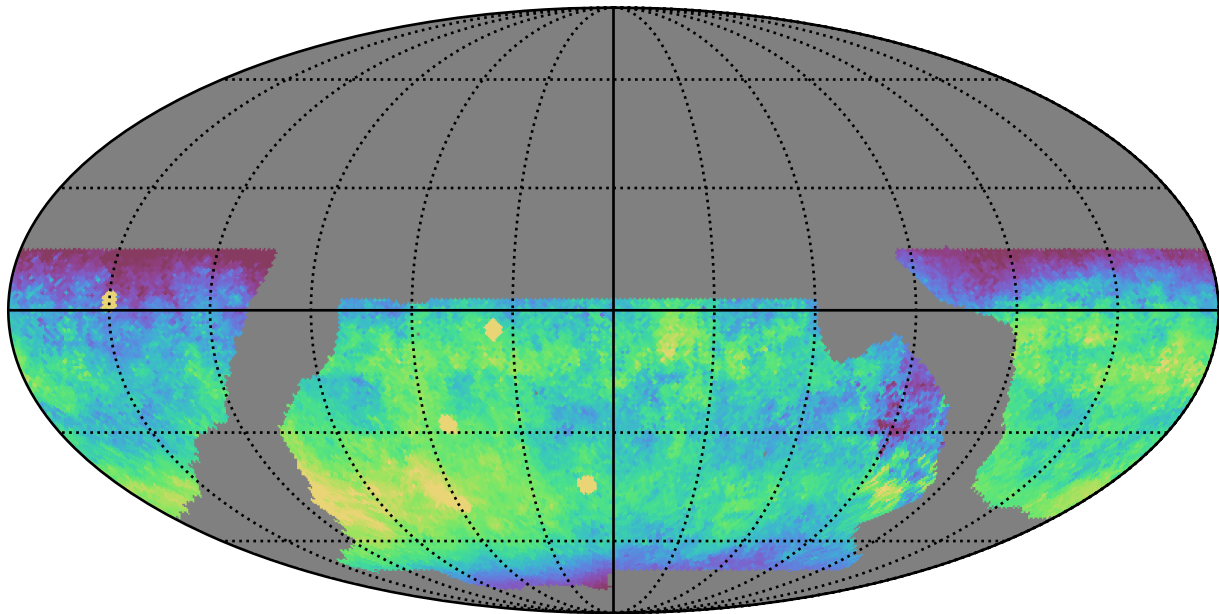
baseline_v2.0_10yrs WFD y band: Median skyBrightness
