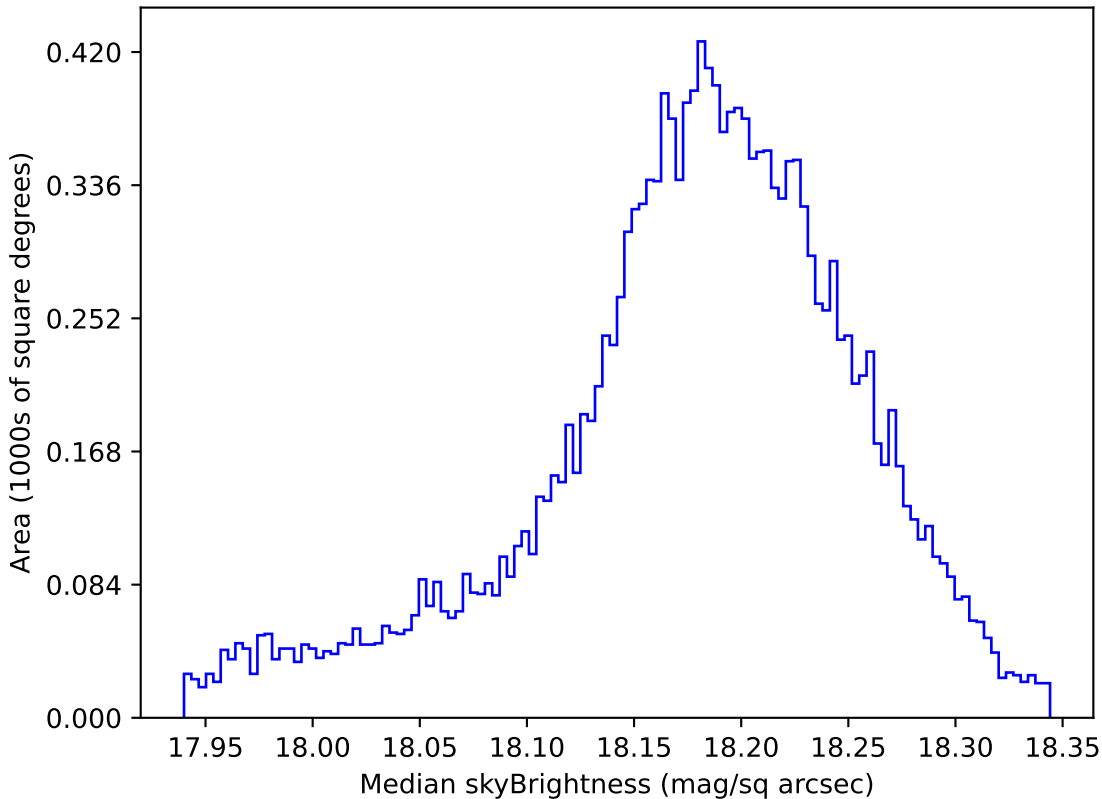
baseline_v2.0_10yrs WFD y band: Median skyBrightness
