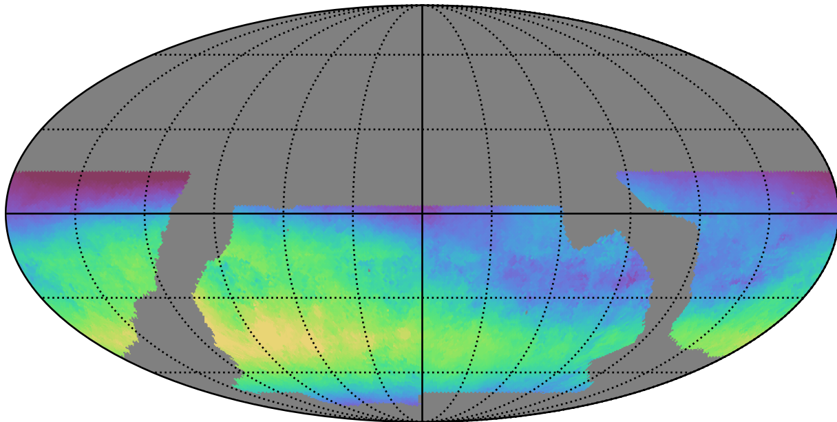
baseline_v2.0_10yrs WFD u band: Median skyBrightness
