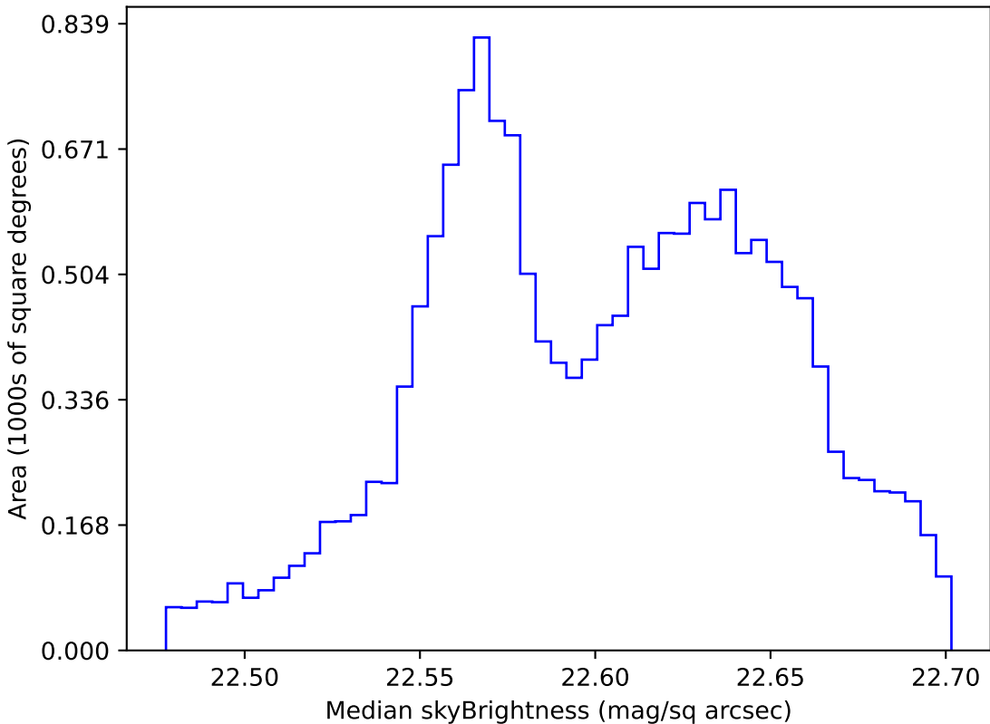
baseline_v2.0_10yrs WFD u band: Median skyBrightness
