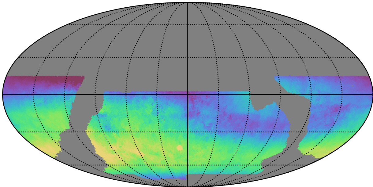
baseline_v2.0_10yrs WFD r band: Median skyBrightness
