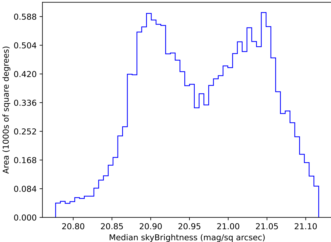
baseline_v2.0_10yrs WFD r band: Median skyBrightness
