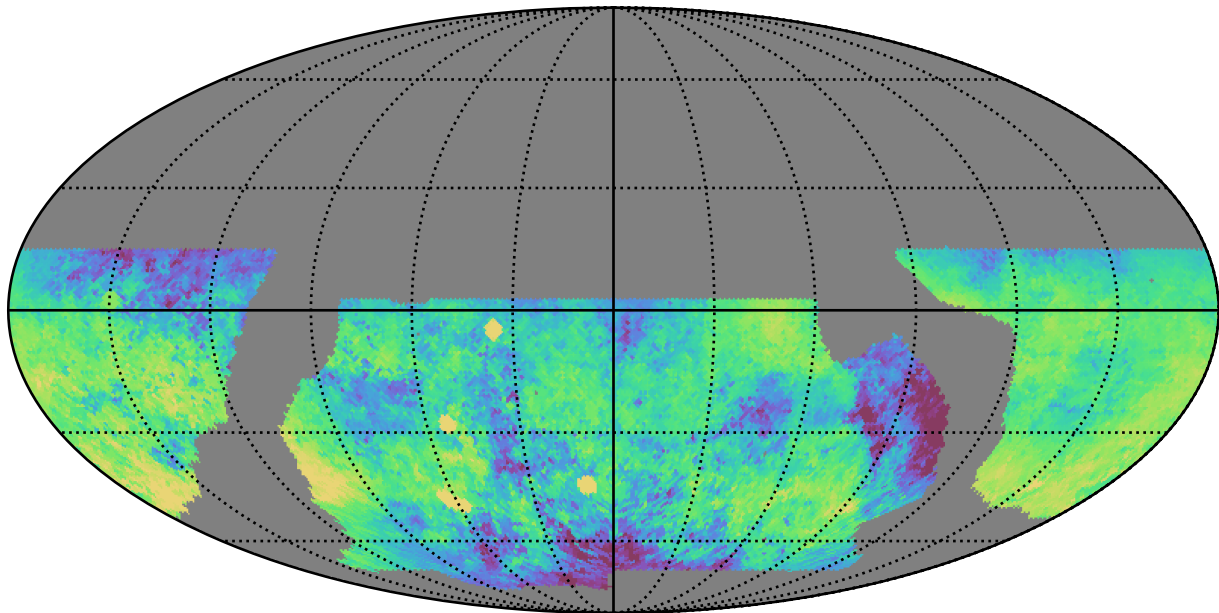
baseline_v2.0_10yrs WFD i band: Median skyBrightness
