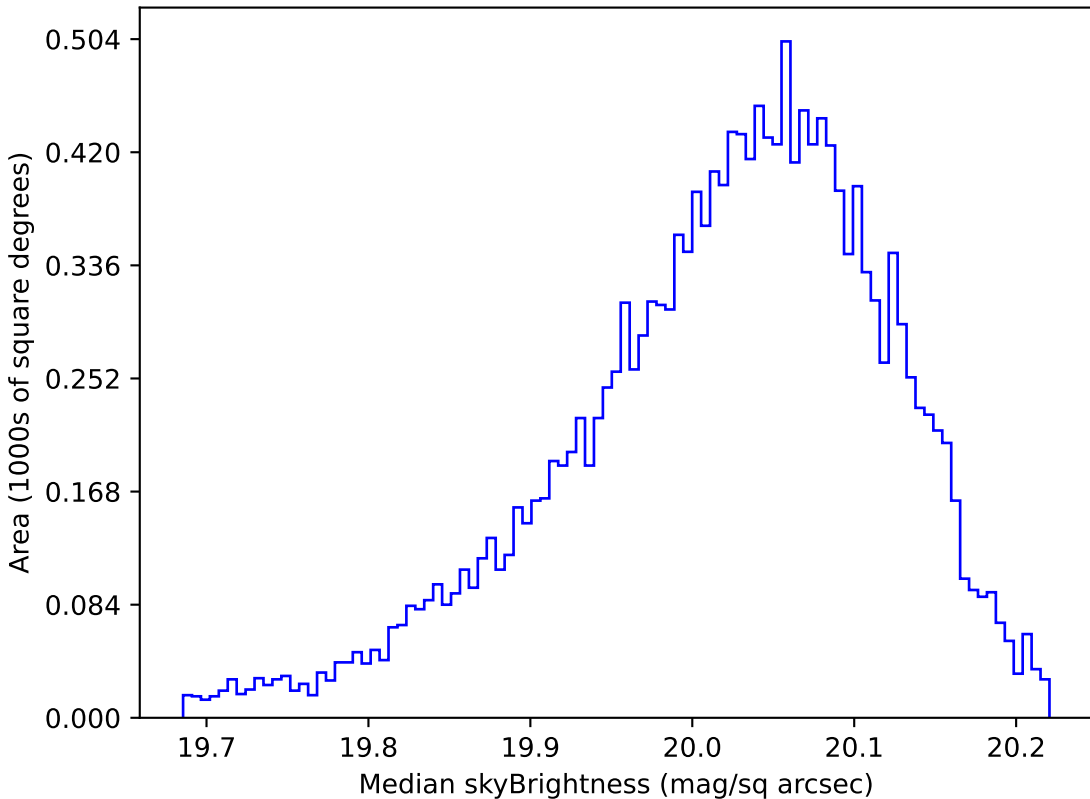
baseline_v2.0_10yrs WFD i band: Median skyBrightness
