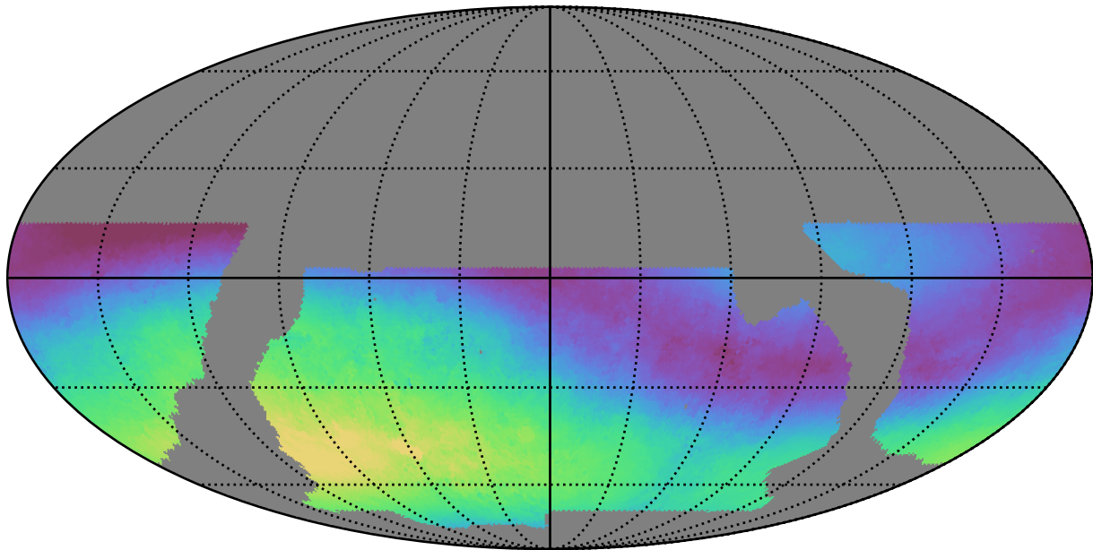
baseline_v2.0_10yrs WFD g band: Median skyBrightness
