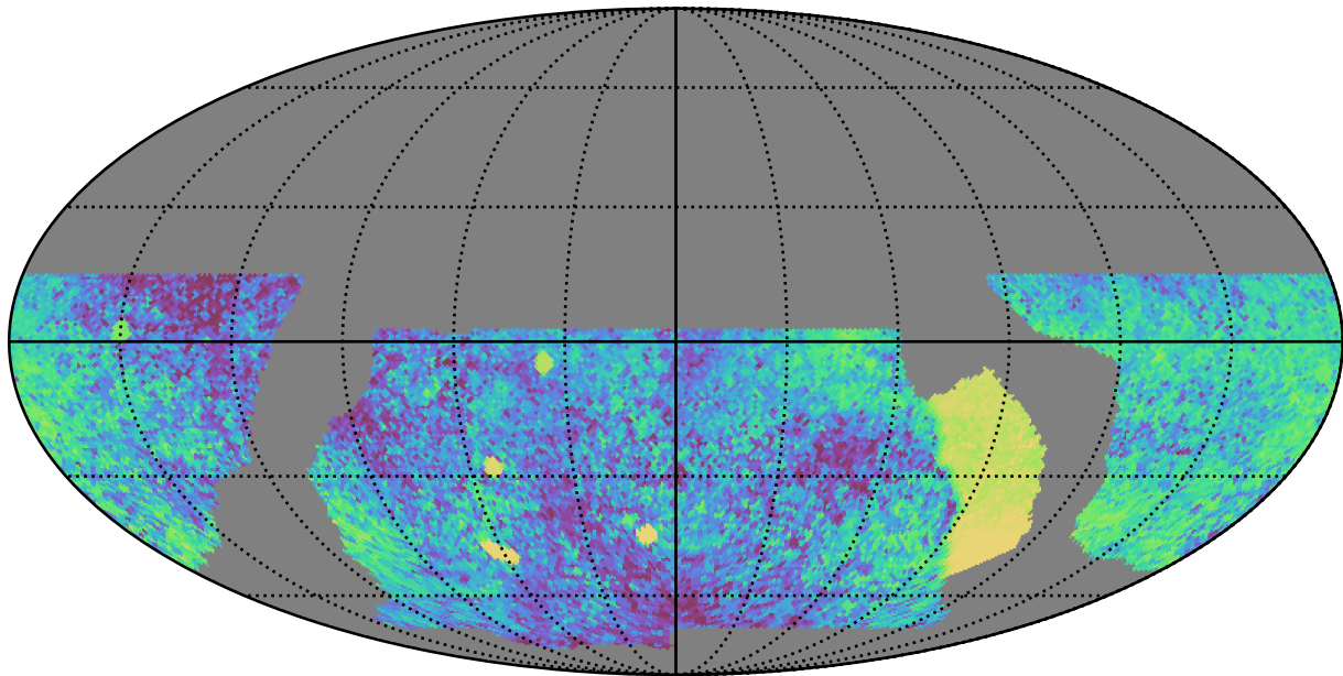
baseline_v2.0_10yrs WFD all bands: Median skyBrightness
