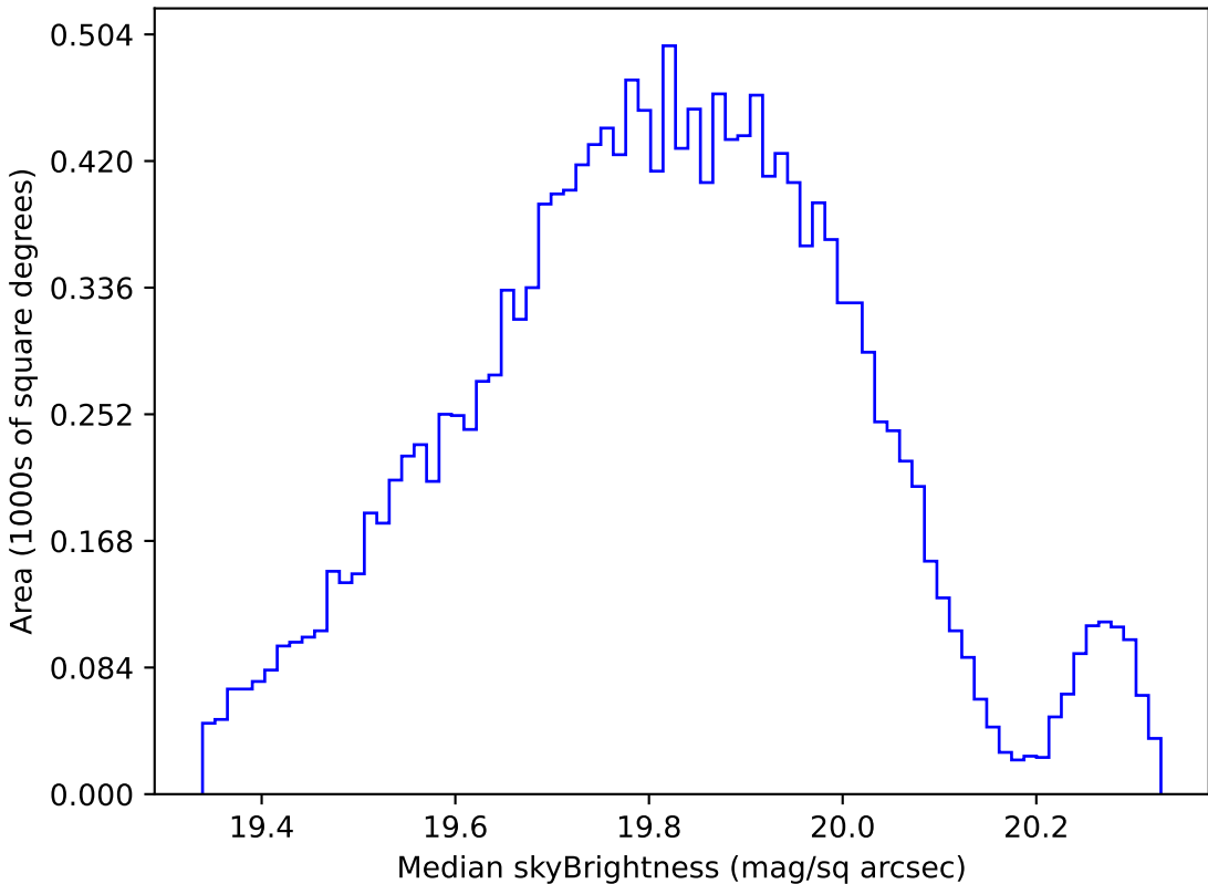
baseline_v2.0_10yrs WFD all bands: Median skyBrightness
