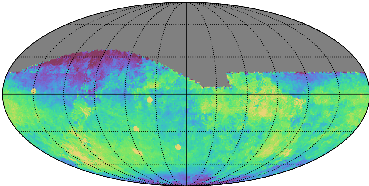
baseline_v2.0_10yrs All sky z band: Median skyBrightness
