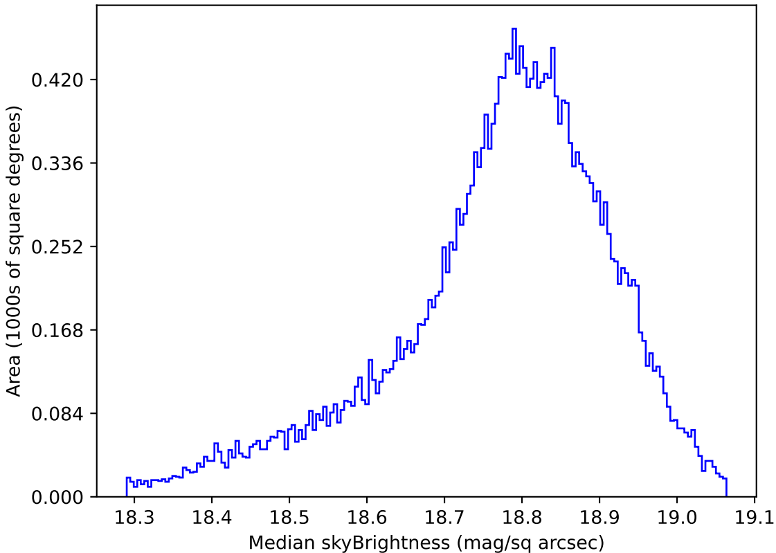
baseline_v2.0_10yrs All sky z band: Median skyBrightness
