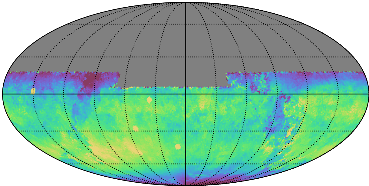
baseline_v2.0_10yrs All sky y band: Median skyBrightness
