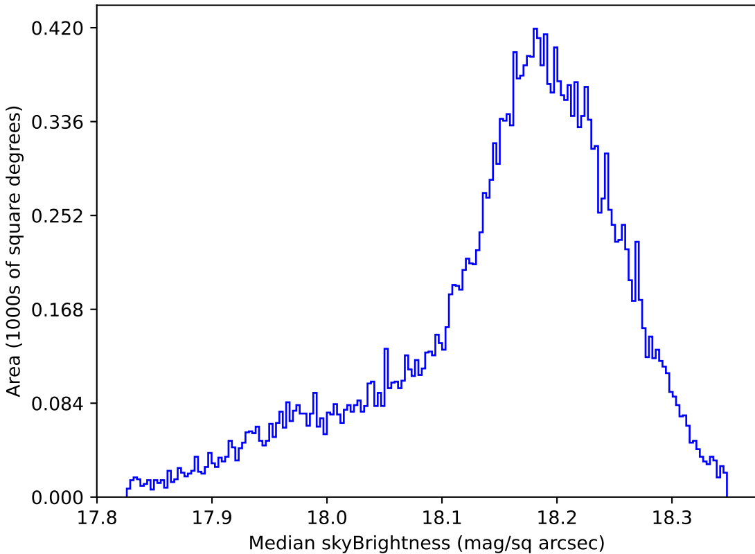
baseline_v2.0_10yrs All sky y band: Median skyBrightness
