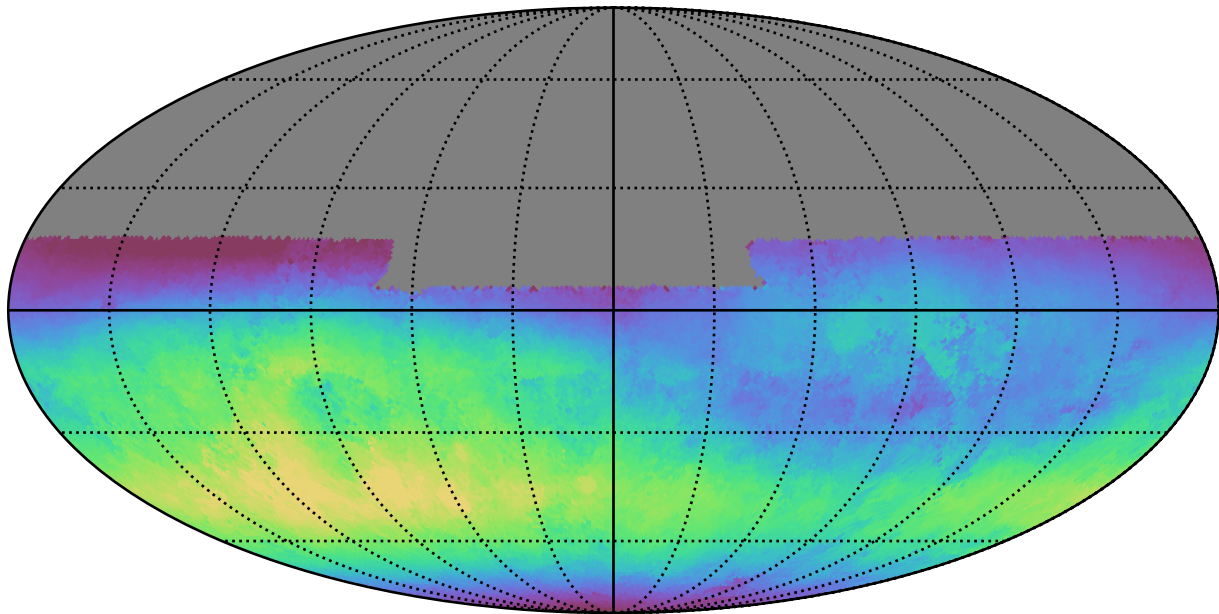
baseline_v2.0_10yrs All sky u band: Median skyBrightness
