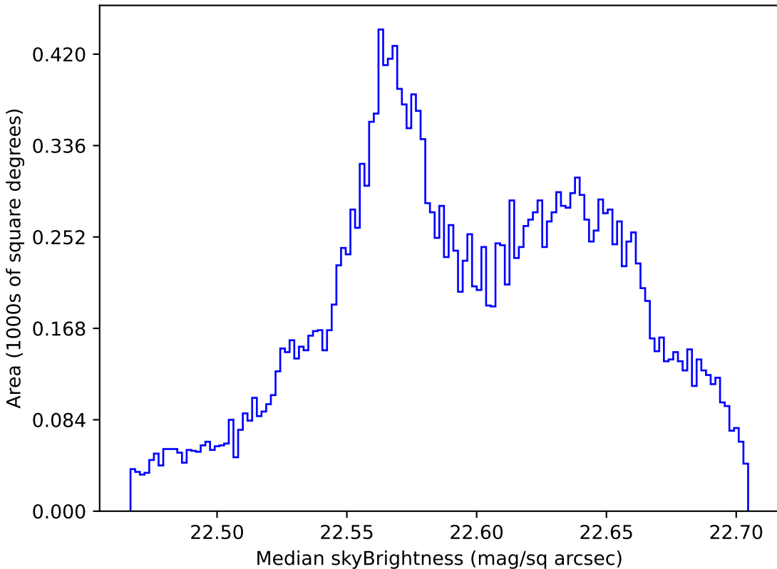
baseline_v2.0_10yrs All sky u band: Median skyBrightness
