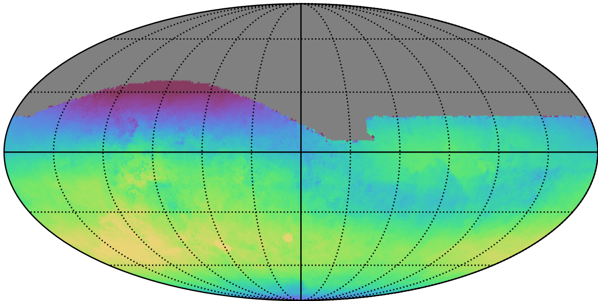
baseline_v2.0_10yrs All sky r band: Median skyBrightness
