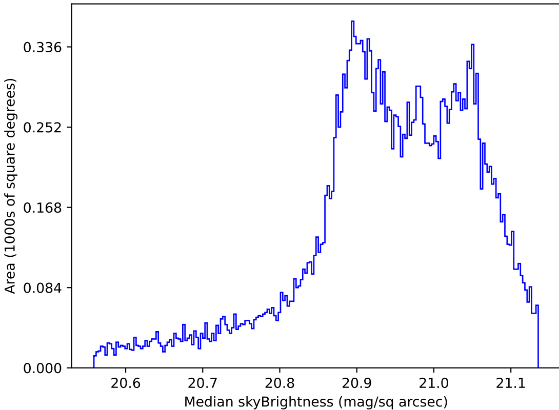
baseline_v2.0_10yrs All sky r band: Median skyBrightness
